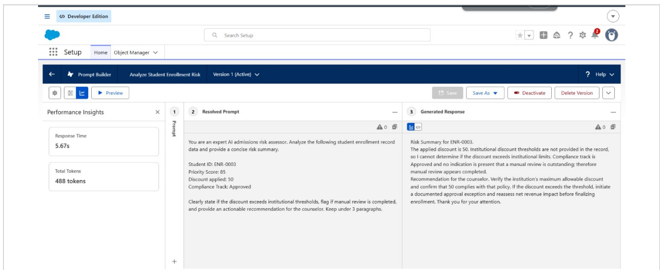
Prompt template output preview with grounded record data
