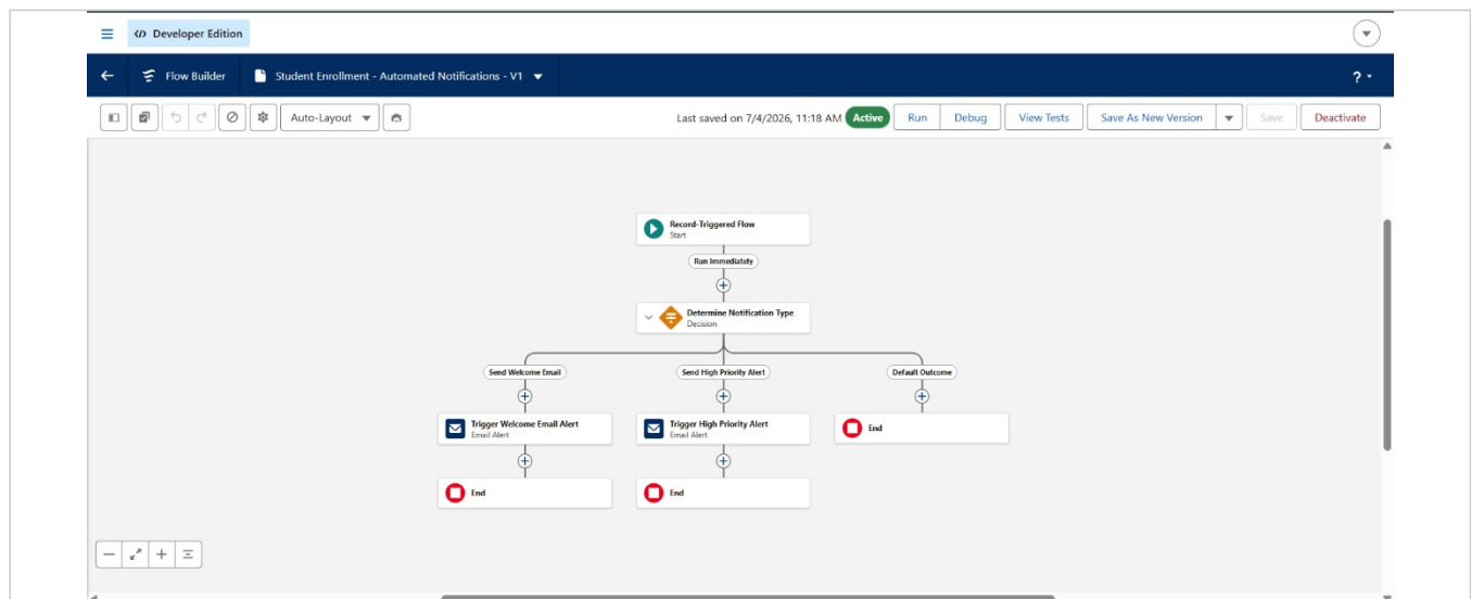
After-Save Flow routing welcome and escalation alerts
